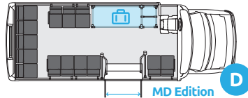
14 Passengers + Luggage rack & 42" Entrance Door
