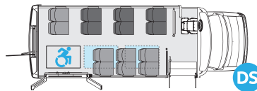
14/12 Passengers + 1 W/C 8 Passengers + 3 W/C
