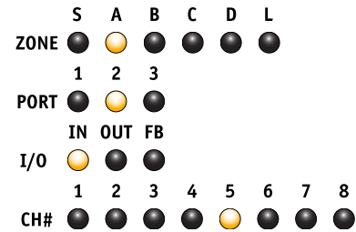
Still displaying A2 Inputs, LED #5 is on only when the ignition switch is in its momentary Start position. As soon as the engine starts, LED #2 (Starter Lockout Signal) comes on and remains on until the engine is switched off.
