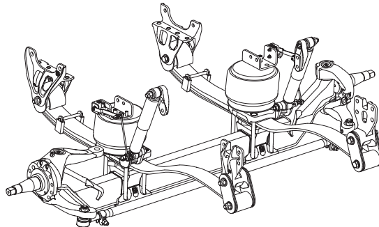
FIGURE 2-2 AIRTEK® Air Suspension System with STEERTEK Axle for Blue Bird All American Buses Capacity: 14,600 pounds
