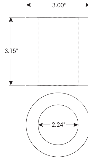
Steering Arm Receiver
