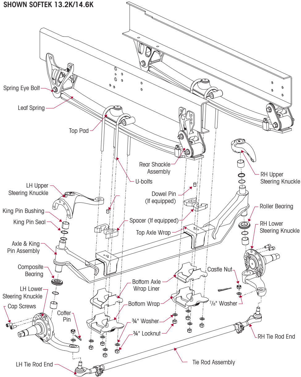
FIGURE 9-41 SHOWN SOFTEK 13.2K/14.6K
