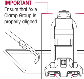
3/4" Clamp Group Locknuts Tightening Torque 285-305 ft. lbs.
