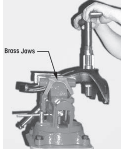
FIGURE 9-70 LOWER STEERING KNUCKLE IN VISE FIGURE 9-71 UPPER STEERING KNUCKLE IN VISE
