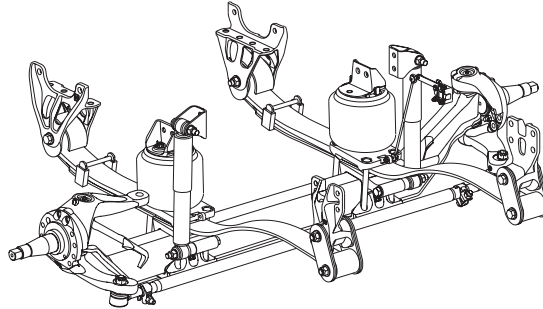
FIGURE 2-1 AIRTEK® Air Suspension System with STEERTEK Axle for Blue Bird Vision Buses Capacity: 10,000 pounds
