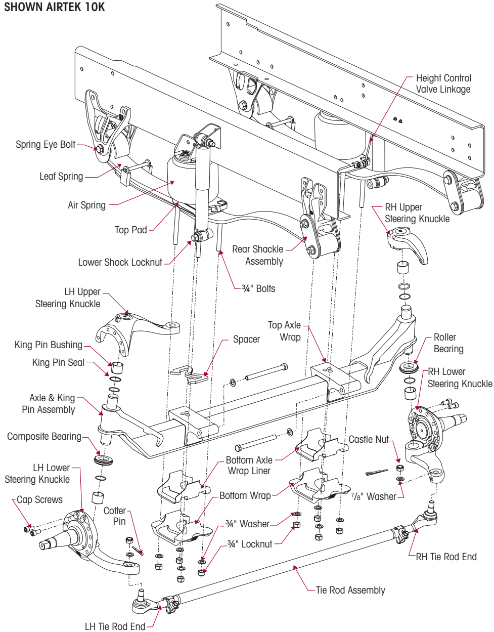
FIGURE 9-40 SHOWN AIRTEK 10K
